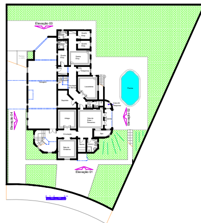
Subsolo A = 342,51 m 2
